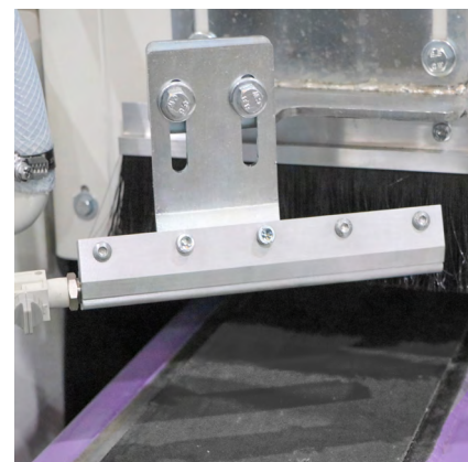
__ air blower: reducing the quantity of splashes outside of the machine
