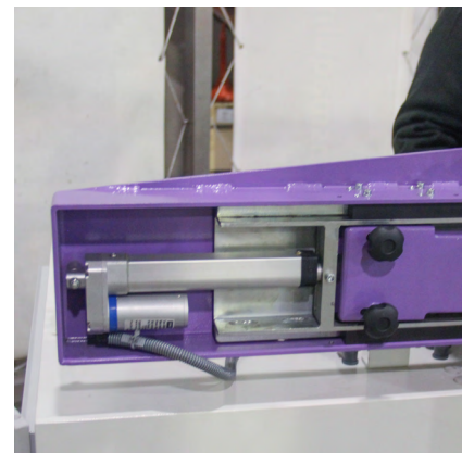
__ pneumatic system for automatic soap applying
